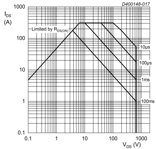
Fig. 17. Forward bias safe operating area
